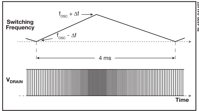
Figure 7. Switching Frequency Jitter (Idealized V_{DRAIN} Waveforms).
